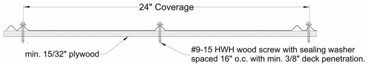
Figure 1: 5V Crimp Panel Fastener Pattern for System 1
